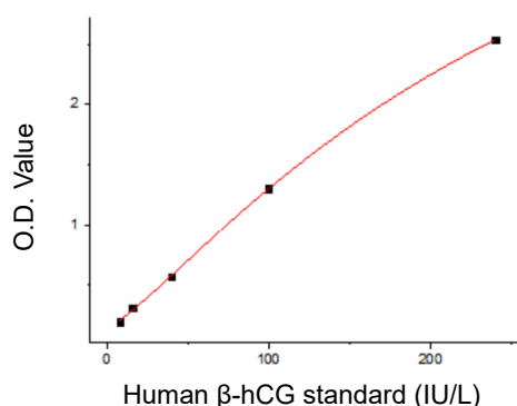
Figure1. Standard Curve of Human β-hCG in 96-well plate assay, data provided for demonstration purposes only. A new standard Curve must be generated for each assay.
